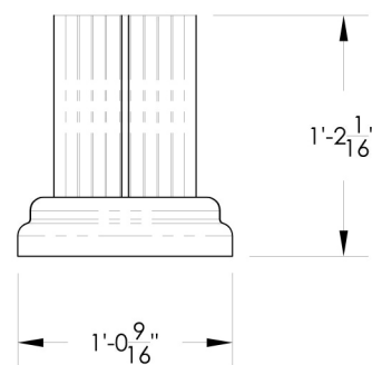
FRONT & SIDE VIEW SHORT PEDESTAL (VOGUEP114)
